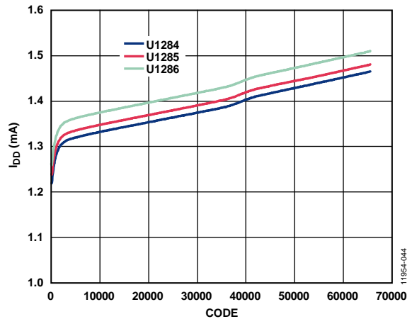
Figure 36. Supply Current ( I_{DD} ) vs. Code
