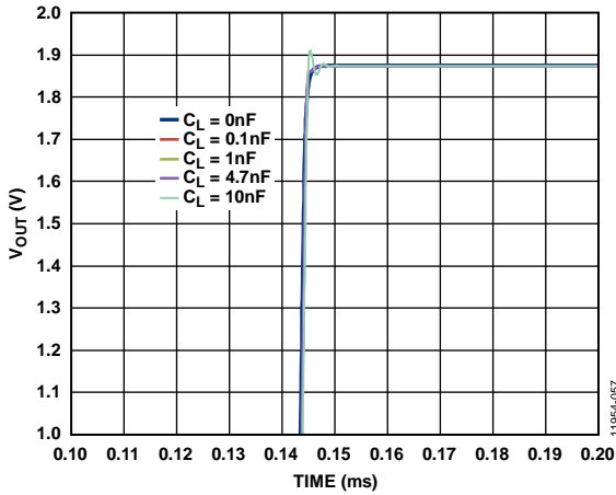
Figure 49. Settling Time vs. Capacitive Load
