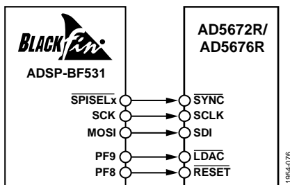
Figure 68. ADSP-BF531 Interface
