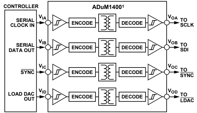
Figure 71. Isolated Interface
