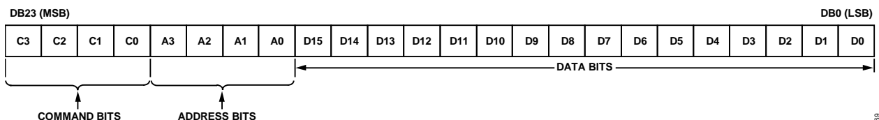
Figure 59. AD5672R Input Shift Register Content
