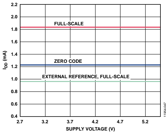
Figure 39. Supply Current ( I_{DD} ) vs. Zero Code and Full Scale
