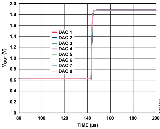
Figure 50. Settling Time, 5.5 V
