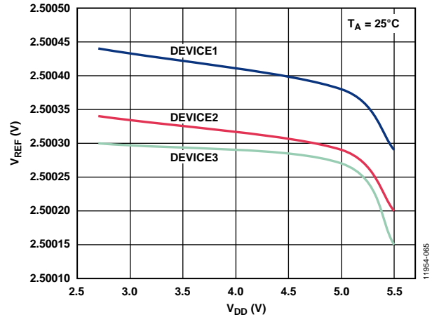
Figure 56. Internal Reference Voltage ( V_{REF} ) vs. Supply Voltage ( V_{DD} )
