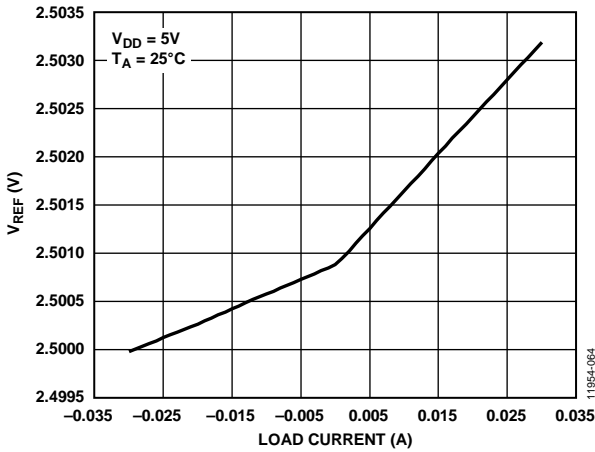
Figure 55. Internal Reference Voltage ( V_{REF} ) vs. Load Current and Supply Voltage ( V_{DD} )
