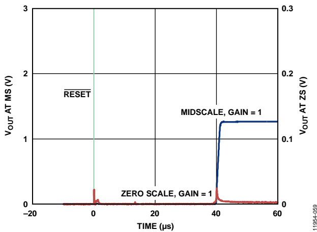
Figure 51. Hardware Reset
