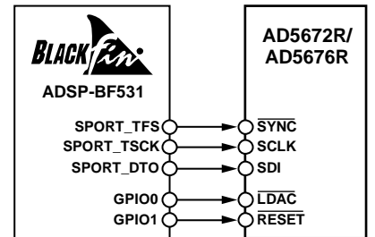
Figure 69. SPORT Interface
