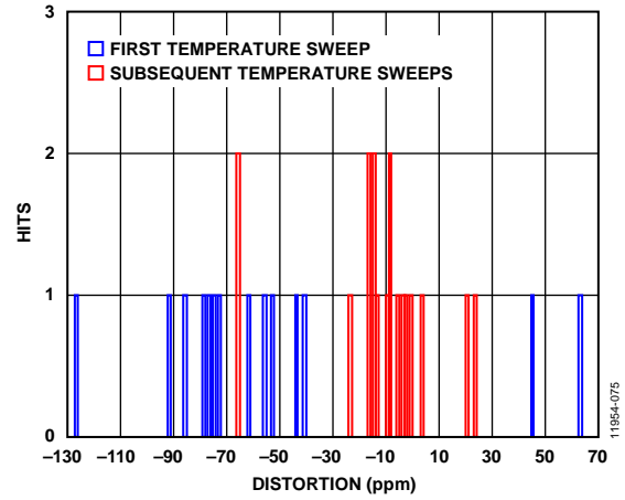
Figure 66. Thermal Hysteresis
