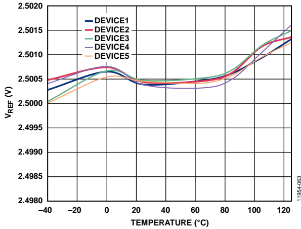
Figure 54. Internal Reference Voltage ( V_{REF} ) vs. Temperature (B Grade)
